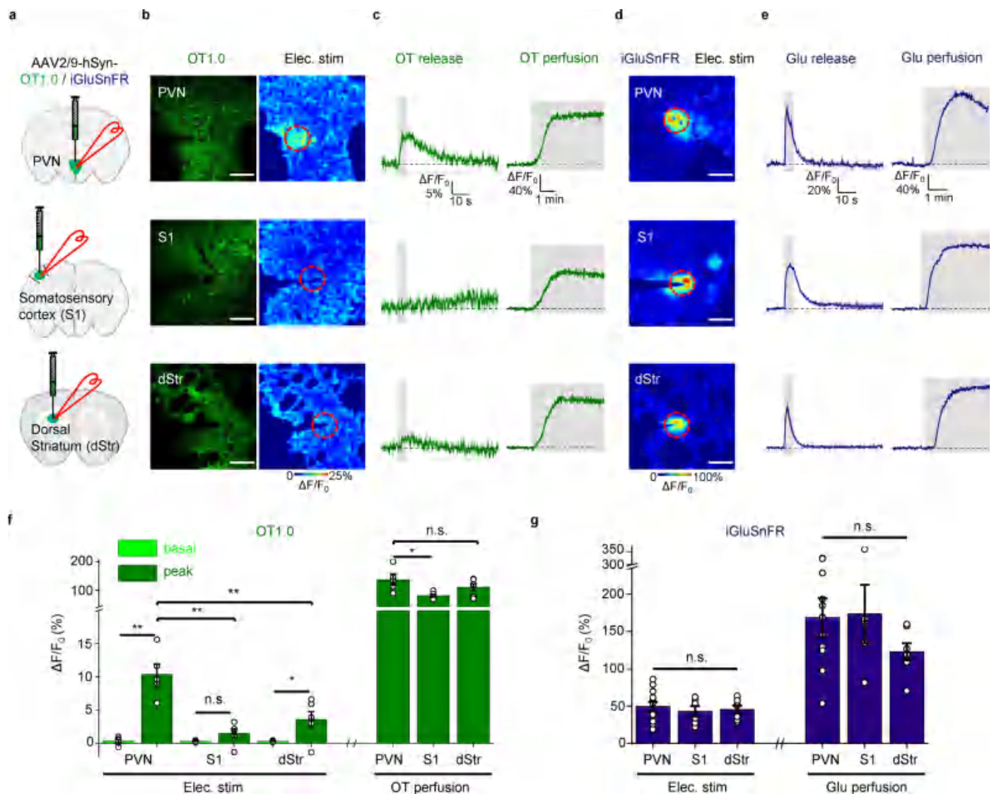
Extended Data Fig. 5 | Electrical stimulation evoked OT and Glutamate release in the PVN, S1 and dStr. a. Schematic illustration depicting the experimental setup for panels (b–g) . b and d. Representative fluorescence images (left) and \Delta F/F_0 pseudocolor images (right) showing the expression and electrical stimulation-induced response of OT1.0 or iGluSnFR in the PVN, S1, and dStr. c and e. Representative traces of electrical stimulation evoked and 100 nM OT or 100 \mu\text{M} Glu perfusion induced OT1.0 or iGluSnFR signals. f and g. Summary of the change in OT1.0 or iGluSnFR fluorescence in response to 100 pulses or ligand application ( n = 5 slices from 4 mice [5/4], 6/3, and 6/3 mice for OT1.0 in the PVN, S1, and dStr, respectively; n = 12 slices from 4 mice [12/4], 6/2, and 7/2 mice for
